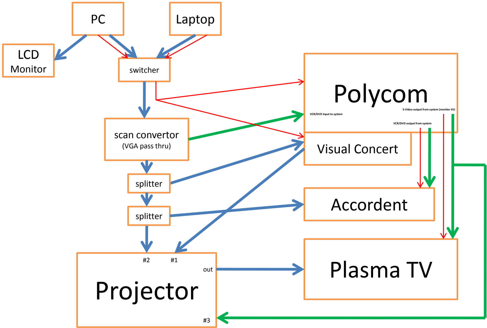
Bldg 970 – Room 1027 A/V wiring diagram
